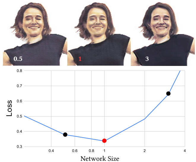
Fig. 5. Impact of network size on the visual quality of results. The loss, y-axis, is computed w.r.t. the output of Jamriška et al. [2019]. The x-axis shows the network size (i.e., number of filters) relative to the best setting we found via hyper-parameter search. Other hyper-parameters are fixed. The middle image (1) depicts the best setting, the left image (0.5) represents setting with half number of filters, and the right image (3) represents setting with three times more filters compared to the middle image. The difference in the visual quality of images, as well as the loss curve, clearly show that there exists a saddle point.
